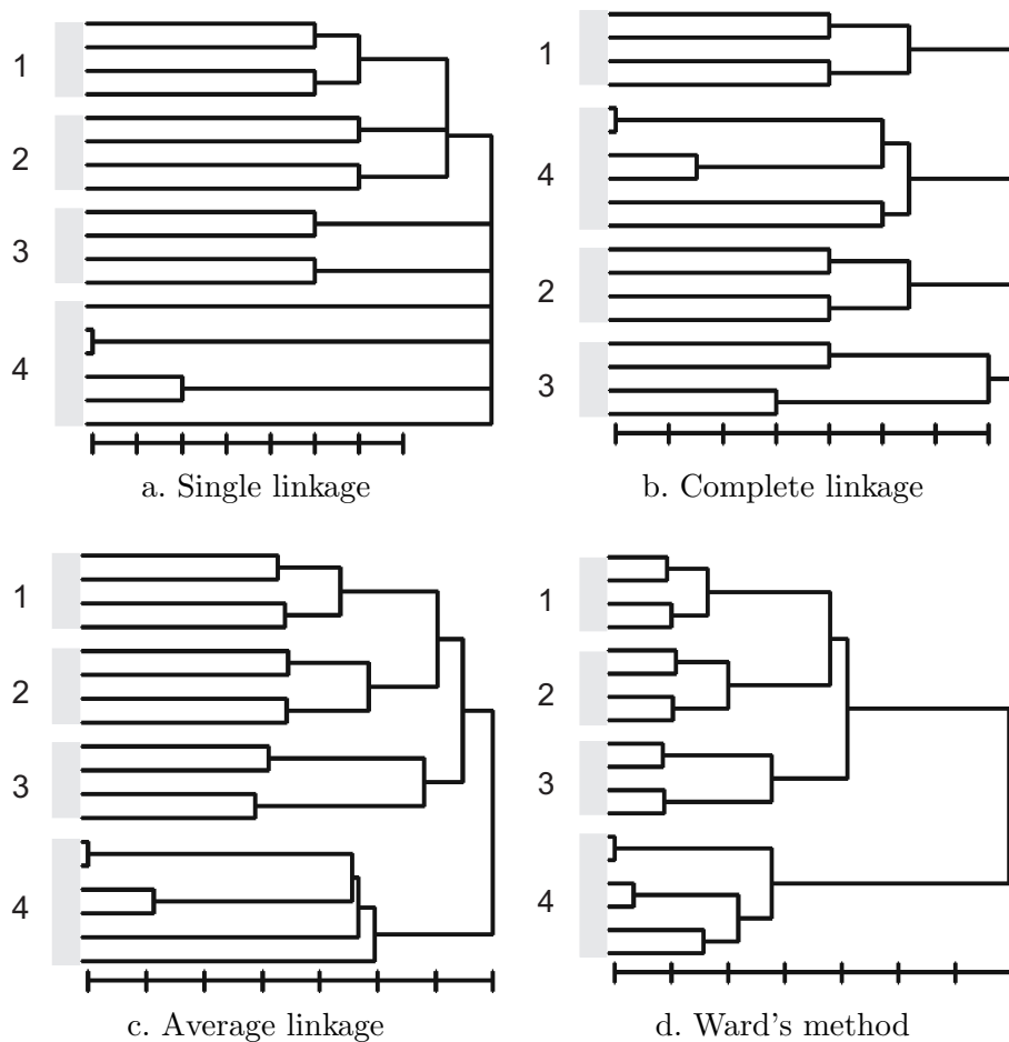
Figure 7. Comparison of four dendrograms from experiment 1: single linkage, complete linkage, average linkage, and Ward method.
